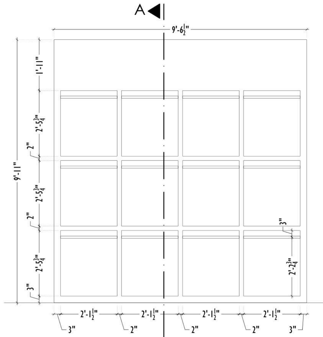
ELEVATION A'◀
